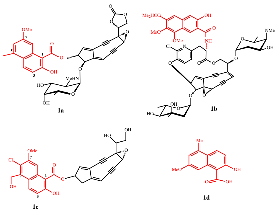
Fig. 1. Structurally diverse chromophore of: (a) NCS (b) kedarcidin (c) N1999A2 and (d) naphthoic acid moiety of NCS. Naphthoic moieties are highlighted in red. (For interpretation of the references to color in this figure legend, the reader is referred to the web version of this article.)
